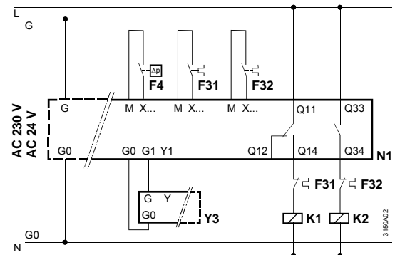
Schaltplan 6:
